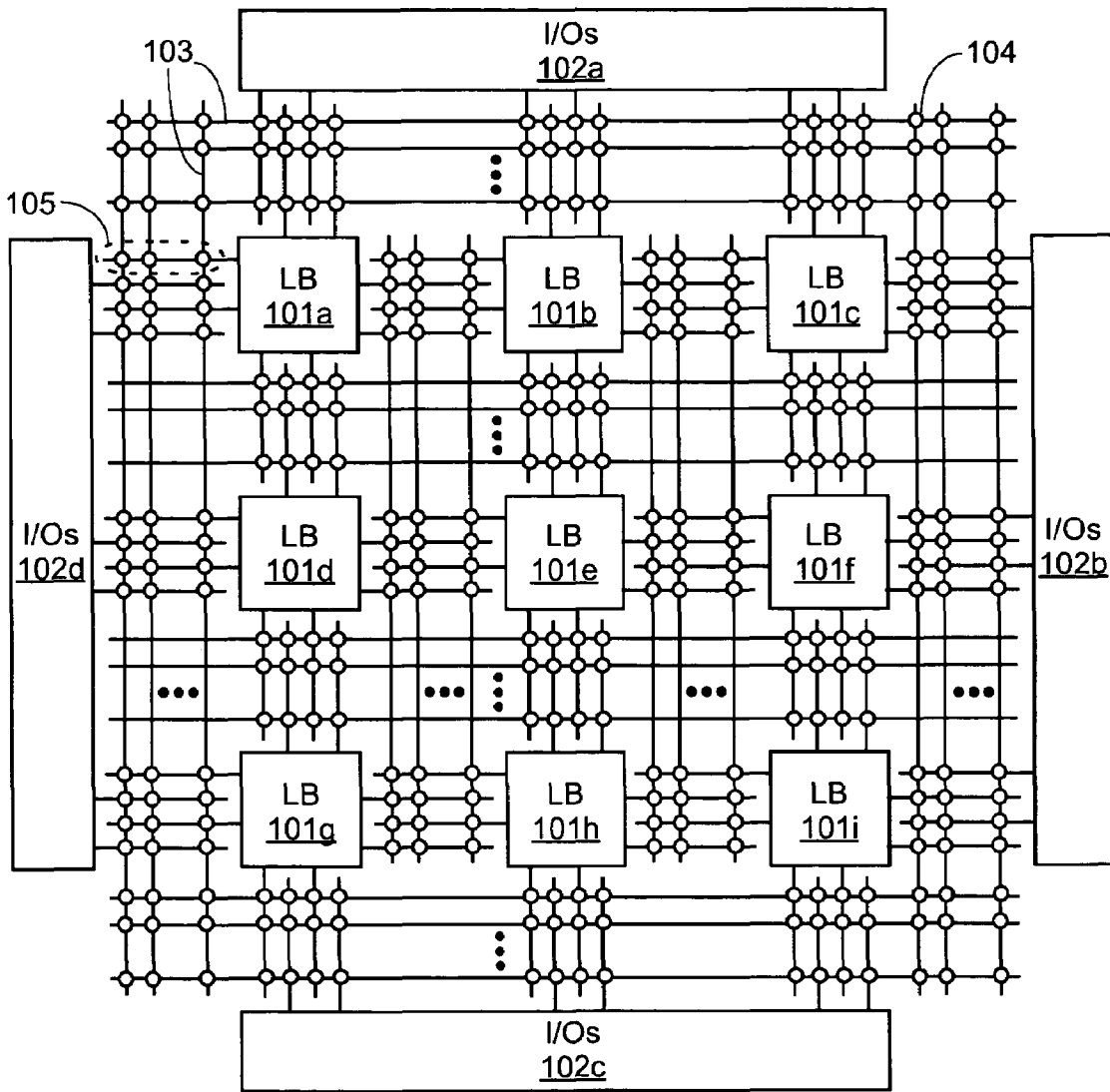
FIG. 1 (Prior Art)
